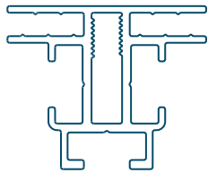
RAPit DOUBLE 40 compact
