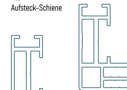
FitFRAME Basis-Schiene 30x53
