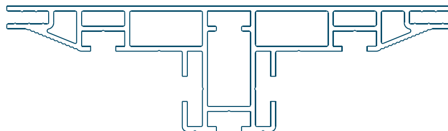
FitFRAME duo160 compact
