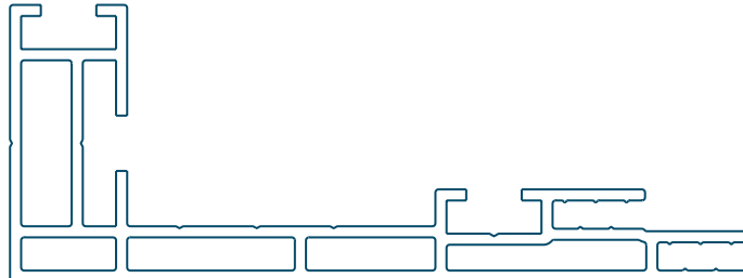
FitFRAME lightbox120
