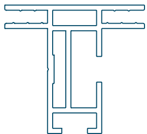
FitFRAME duo50 compact
